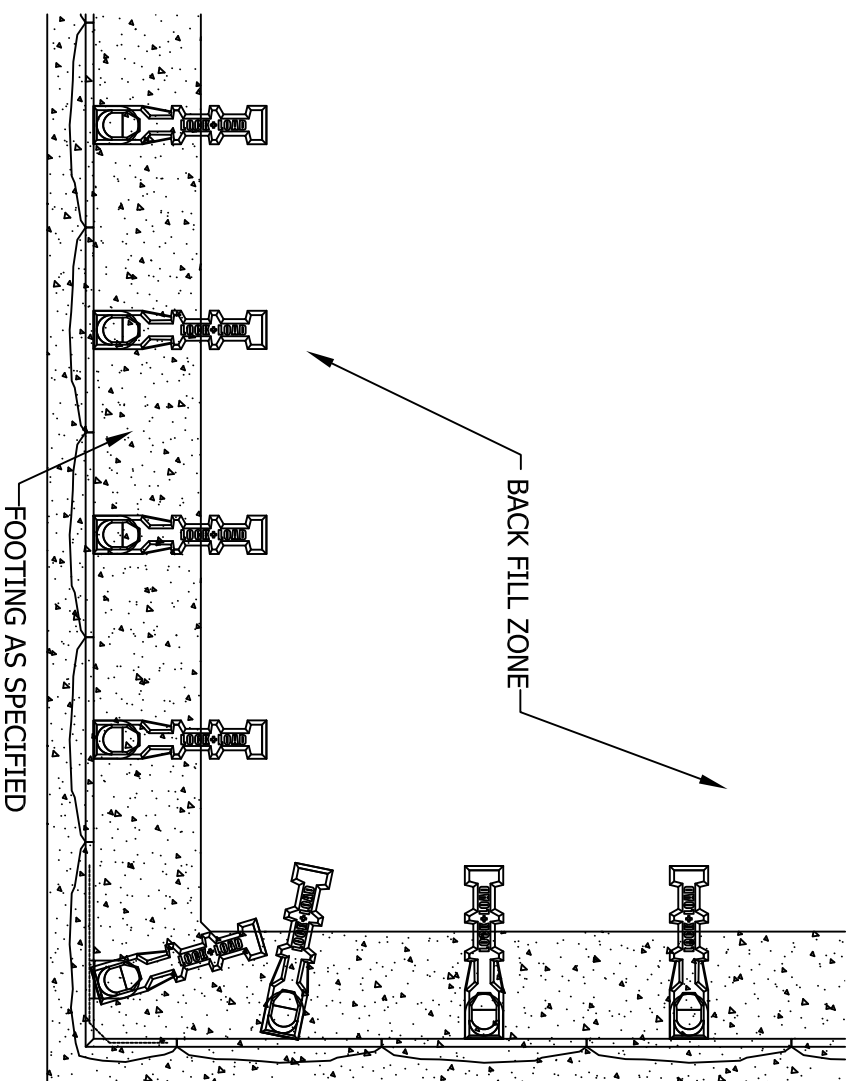
PLAN VIEW FOUNDATION PAD CORNER
