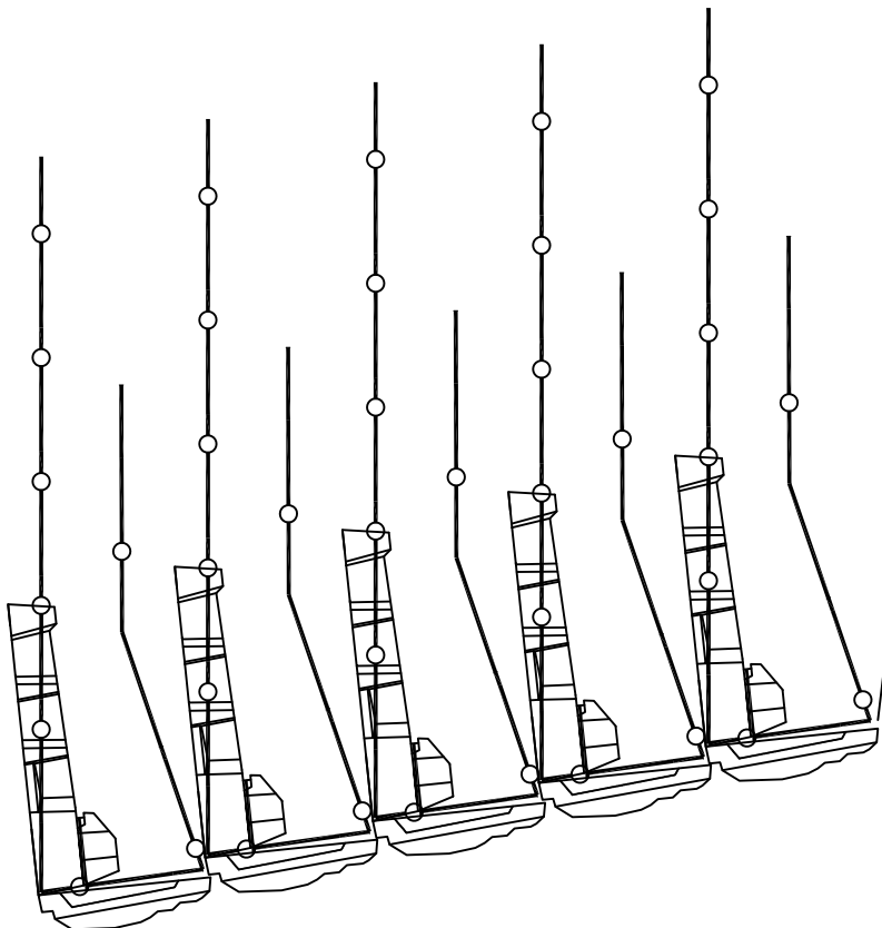
1:5 WALL BATTER
